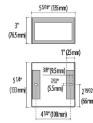
Fascade Cover
